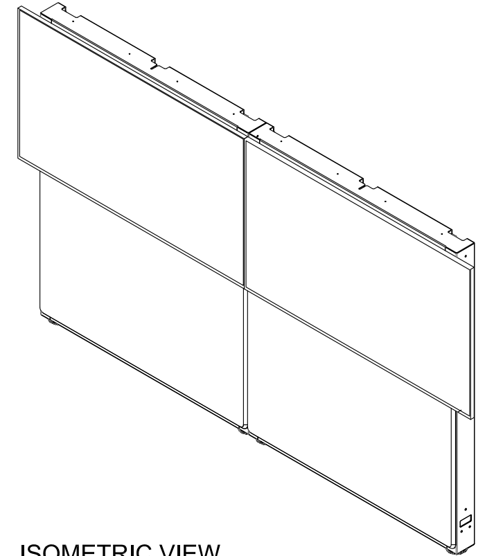
ISOMETRIC VIEW Model shown with 2 x LG55UH5J-H
